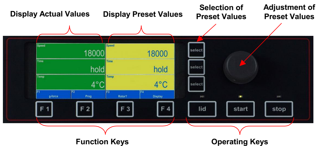
Operating Panel of HiGen 18
